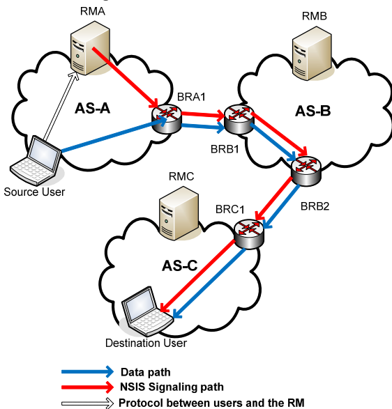
Fig. 3 – NSIS without HyPath support
