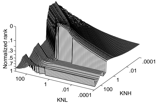
Figure 5.14: A representation of the cost surface associated with the formulation including goal information.
