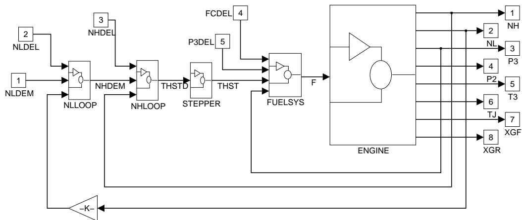
Figure 5.7: The SIMULINK model of the system.
