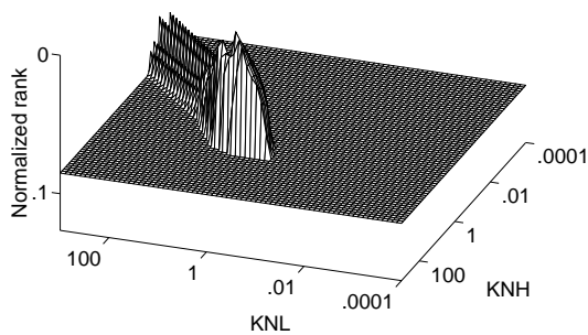
Figure 5.10: The cost surface associated with the settling time of the closed-loop step response.
