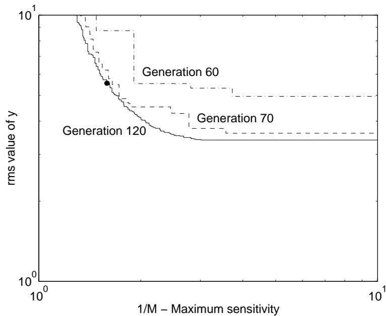
Figure 5.5: Maximum sensitivity versus output variance ( u_{\text{rms}} \leq 10 and 1/D \leq 10 ).
