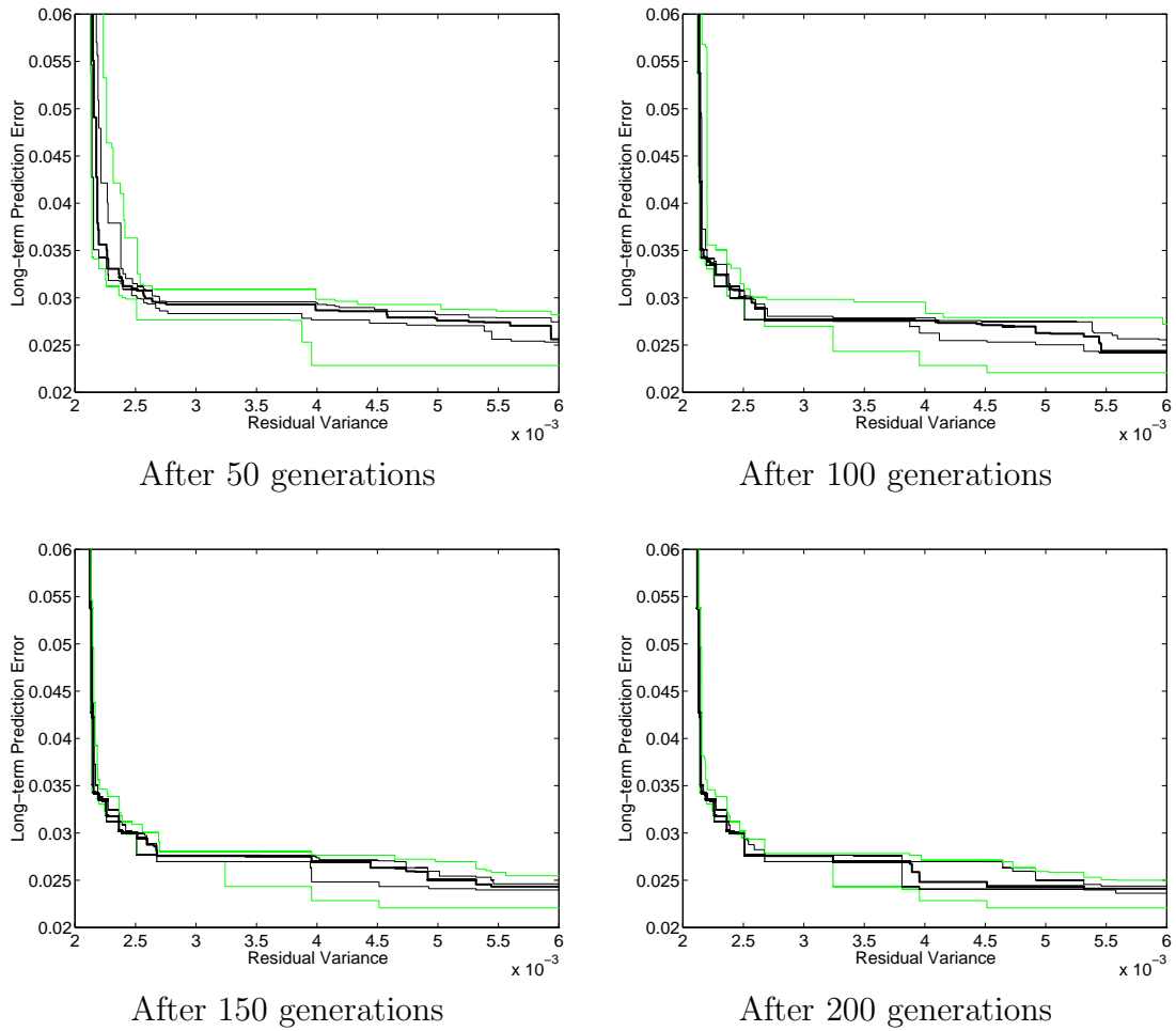
Figure 6.6: Evolution of low-residual variance and low long-term prediction error models (13 runs).
