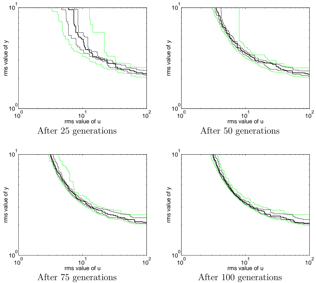
Figure 5.3: Evolution of the noise sensitivity trade-off (13 runs).
