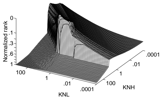
Figure 5.8: The cost surface associated with the maximum pole magnitude of the closed-loop system.
