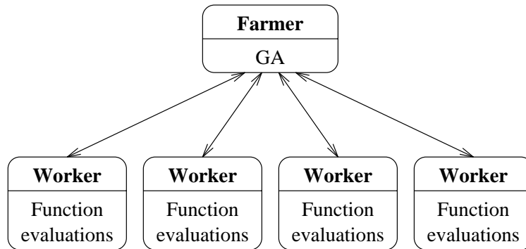
Figure 2.5: Farmer-worker implementation of the GA.
