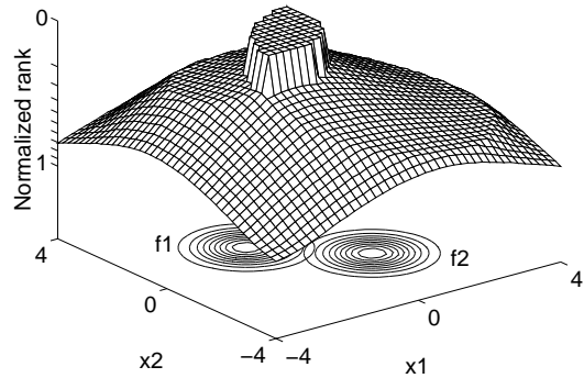
Figure 4.6: The effect of making both f_1 and f_2 into hard objectives (same goals).
