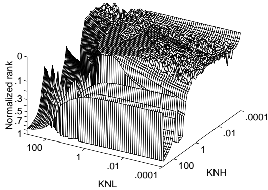
Figure 5.12: A representation of the cost surface associated with the Pareto-based formulation in the absence of preference information.
