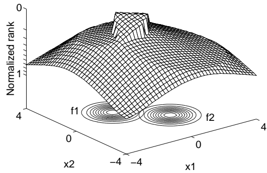
Figure 4.4: The effect of specifying two goals with the same priority.
