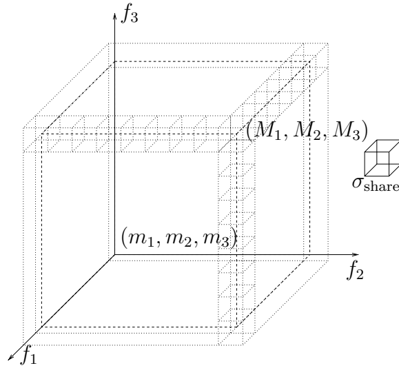
Figure 4.10: Sampling area A . Each point is \sigma_{\text{share}} apart from each of its neighbours ( \infty -norm).
