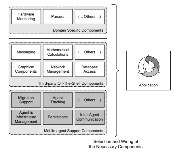
Figure 3 – Applications are developed by wiring different kinds of software components
