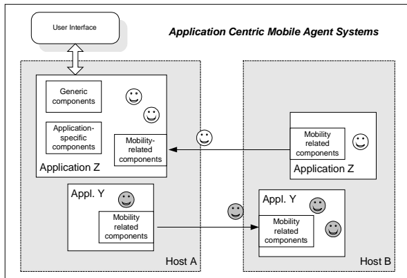
Figure 2 – Application-centric mobile agent systems
