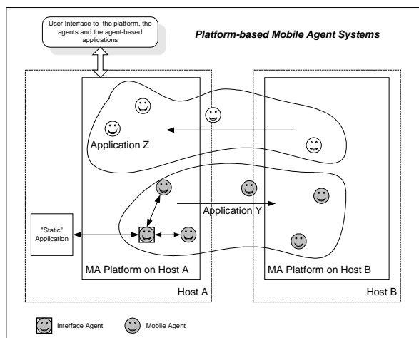
Figure 1 – Platform-based mobile agent systems
