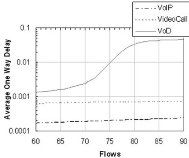
Figure 11. One-way delay
