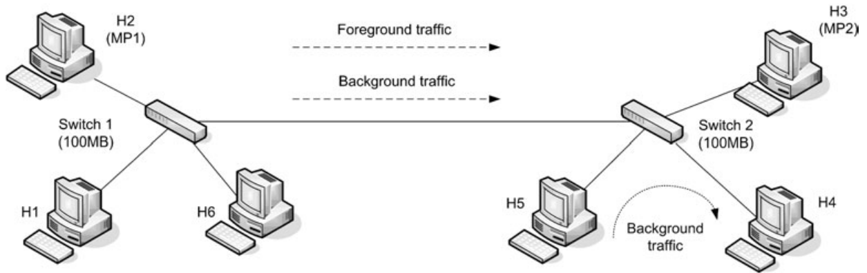
Figure 10. Testbed scenario
