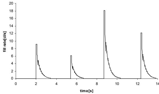
Figure 11. Controller output.
