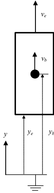
Figure 3. Ball and elevator coordinate system.
