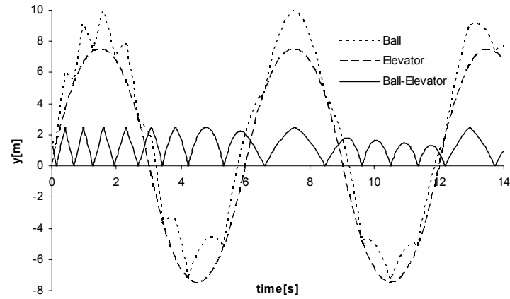
Figure 5. Ball and elevator position.
