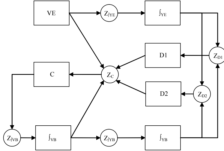
Figure 4. Bouncing ball and elevator block diagram.
