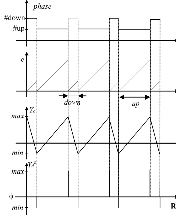
Figure 2. Triangular wave generator trajectories.
