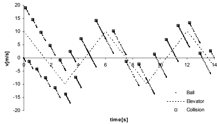
Figure 6. Ball and elevator velocity.
