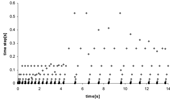
Figure 7. Time steps for ball position integrator.
